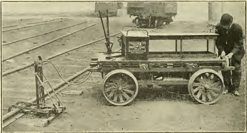
Fig. 4. Bridge-Gang Car with Power Attachment.
